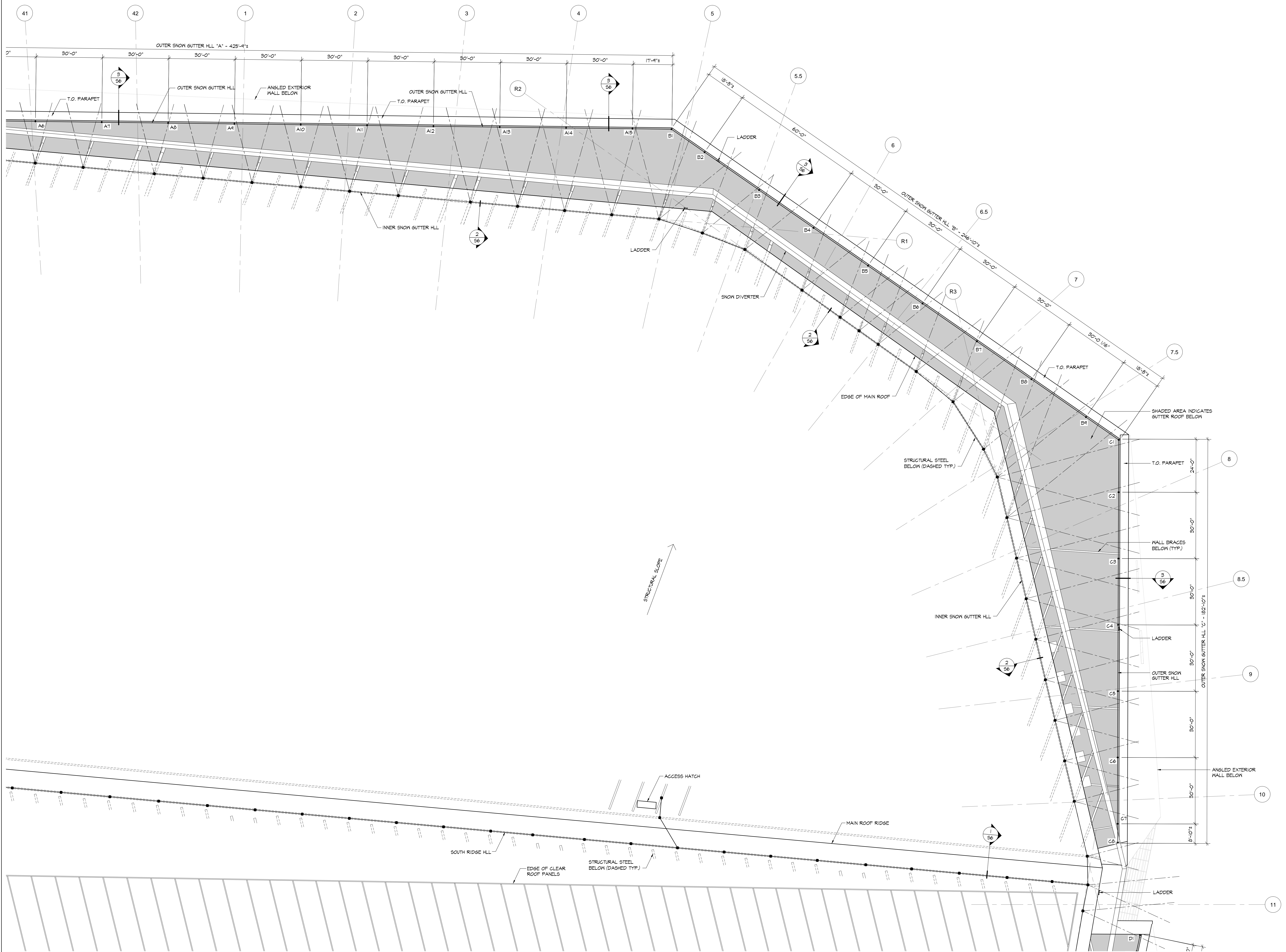
PARTIAL ROOF PLAN 1/16" = 1'-0" NORTH
